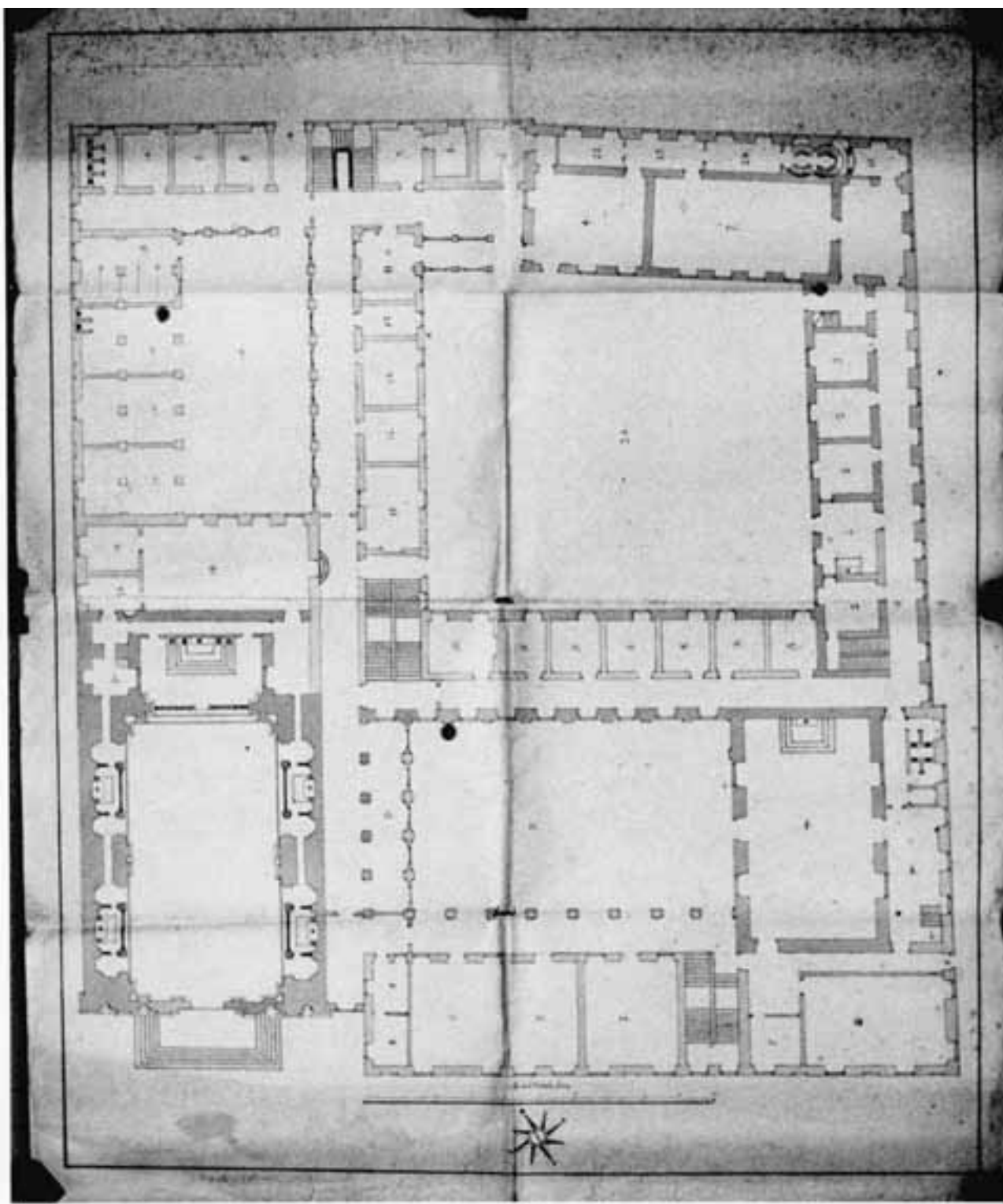
244. Turin, Collegio Vecchio, Plan Nr. 2.
